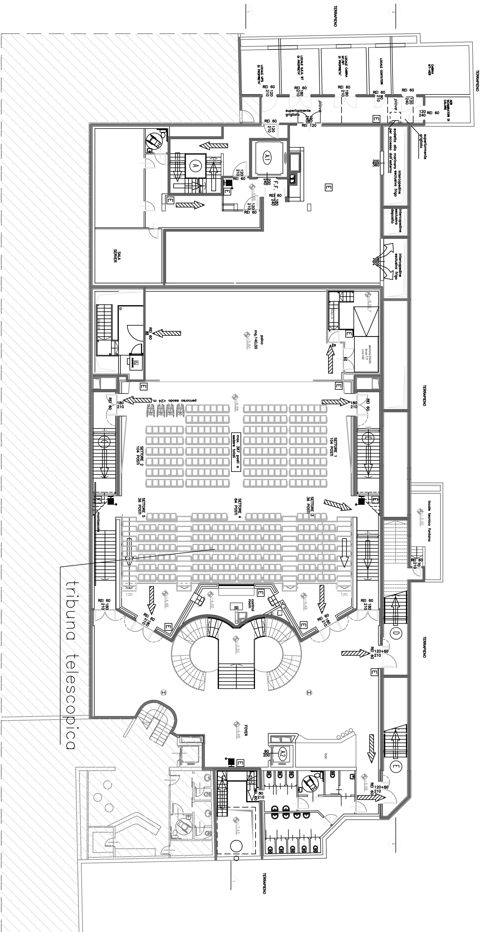
PIANTA PIANO -1
